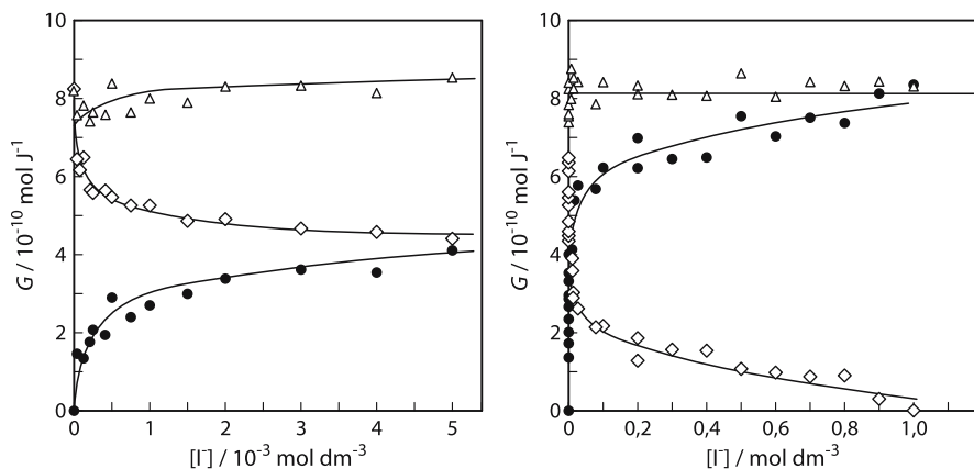
Fig. 2.1. Sonolysis of Ar-saturated water at 321 Hz and an intensity of 170 \text{ W kg}^{-1} . Yields of \text{I}_2 (●), \text{H}_2\text{O}_2 (◇) and \text{I}_2 plus \text{H}_2\text{O}_2 (△) as a function of low concentrations of iodide ( left ) and as a function of high concentrations of iodide ( right ). Source: von Sonntag et al. (1999), with permission
