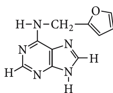
Kinetin
