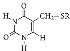
5-cysteinyl- methyluracil
