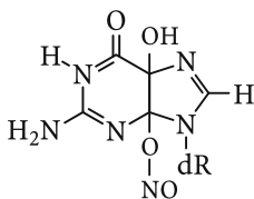
4,5-Dihydro-5-hydroxy-4-(nitrosooxy)-2'-deoxyguanosine
