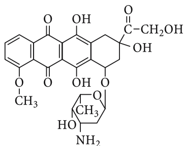
Adriamycin
