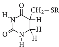
5-cysteinyl-5,6- dihydro-methyluracil
