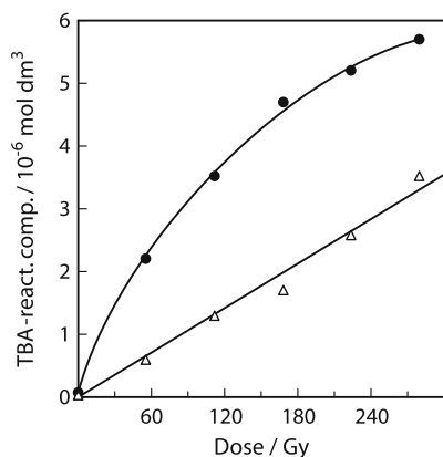
Fig. 12.11. \gamma -Irradiation of DNA ( 1 \times 10^{-3} \text{ mol dm}^{-3} ) in aqueous \text{N}_2\text{O}/\text{O}_2 -saturated solution. Formation of free malonaldehyde (open triangles) and total TBA-active material (filled circles, malonaldehyde plus DNA bound, in malonaldehyde equivalents as regards optical absorption) according to Rashid et al. (1999, with permission)
