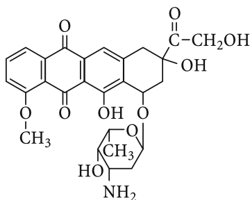
11-Deoxyadriamycin
