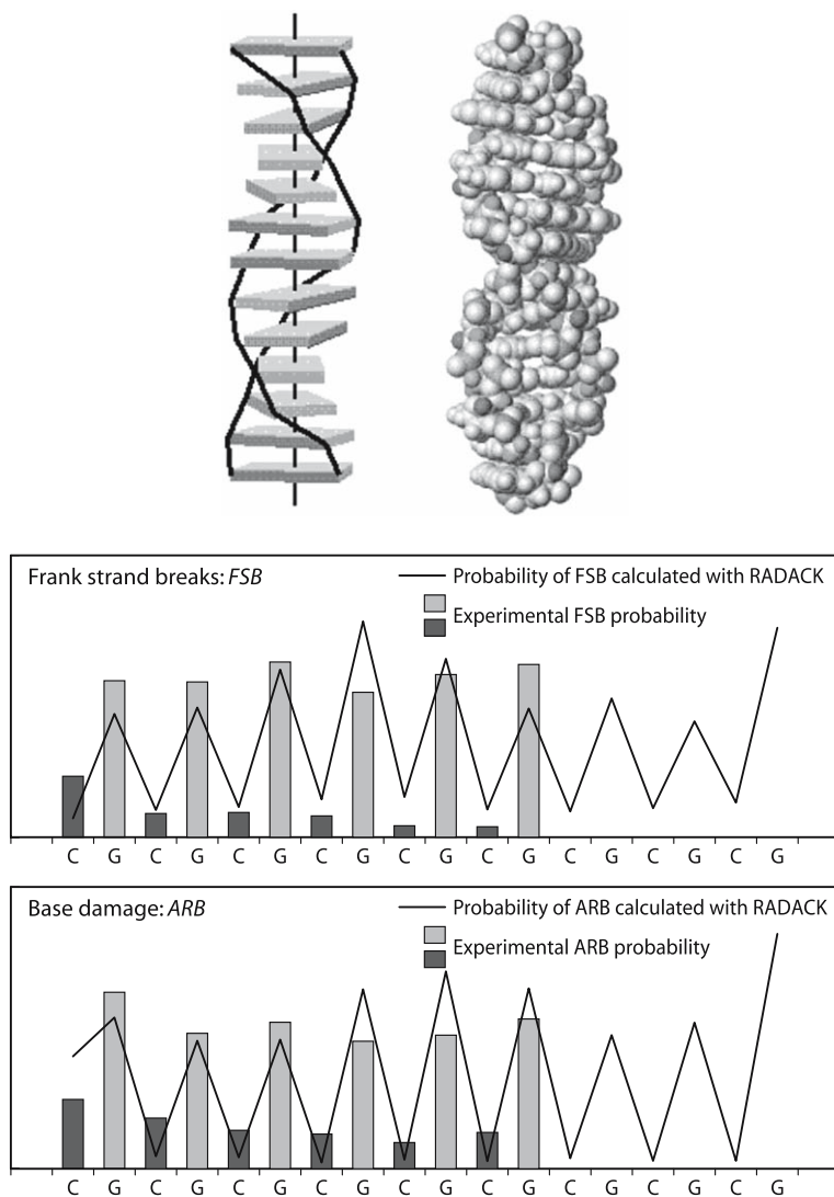
Fig. 12.6. Radiolysis of Z-DNA. Frequency of frank SSBs ( top ) and damaged bases (ALs, bottom ). Solid lines were calculated using RADACK procedure according to Spothem-Maurizot et al. (2003, with permission)
