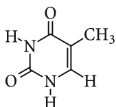
Thymine (Thy)
