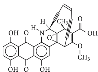
Dynemicin
