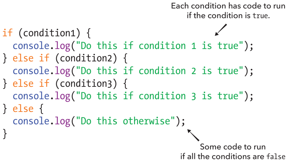
Figure 6-3: Chaining multiple if...else statements
