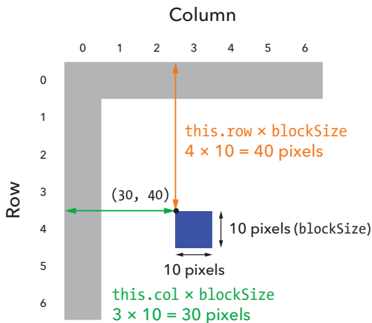
Figure 17-2: Calculating the values for drawing a square
