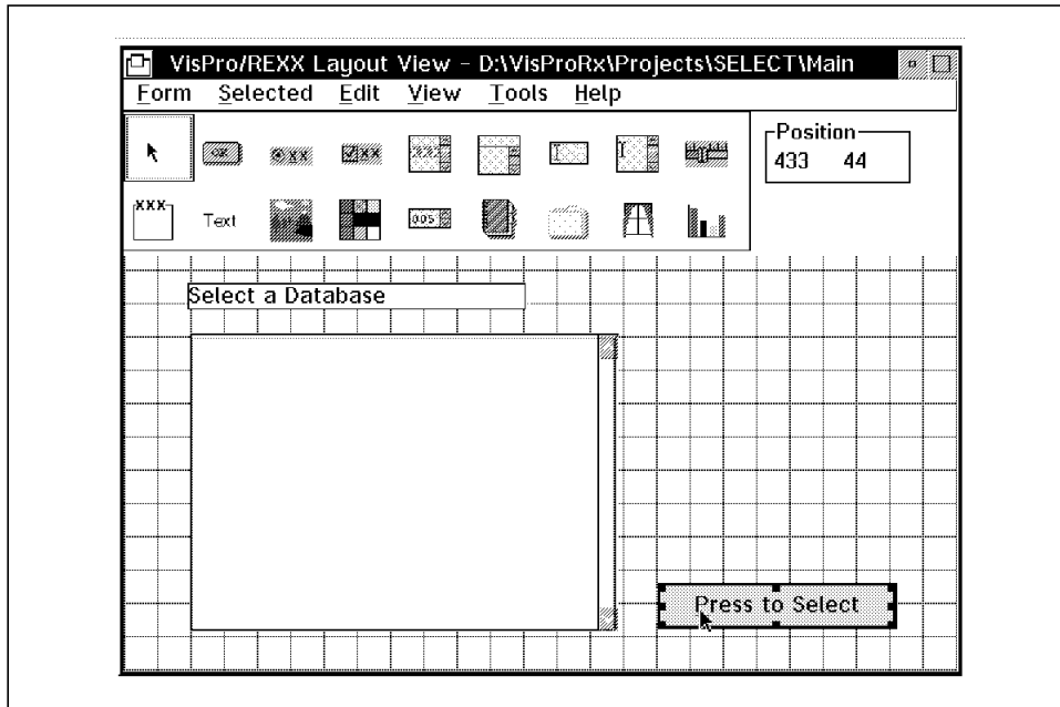
Figure 131. Main Form Layout in VisPro/REXX
