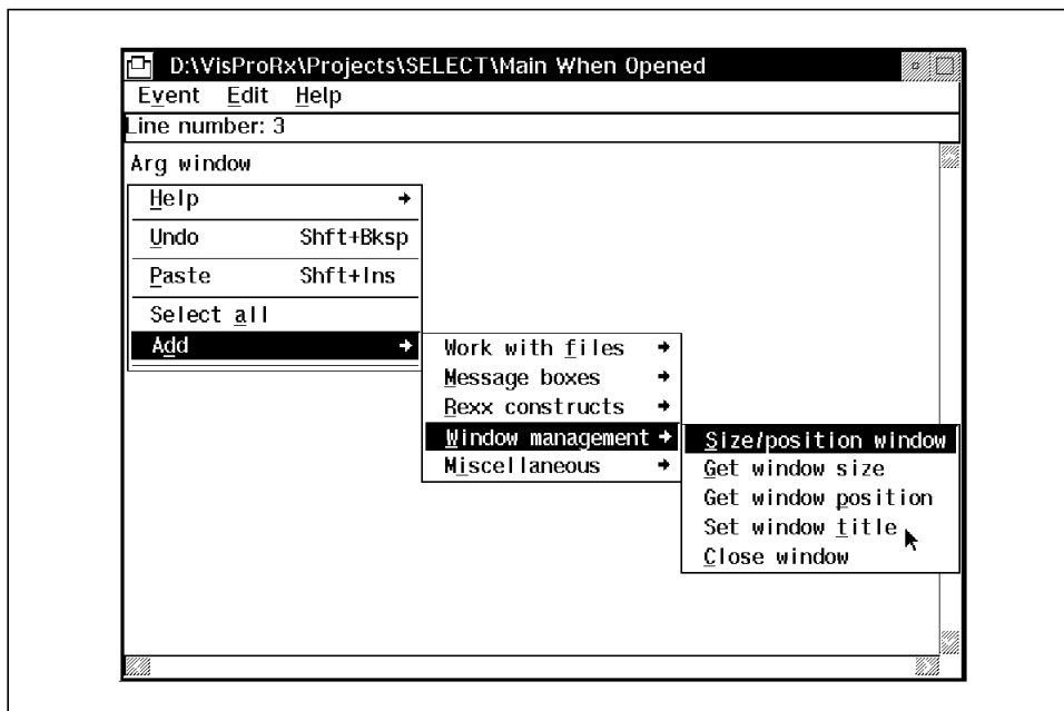
Figure 135. Add Window Management in Code Window in VisPro/REXX
