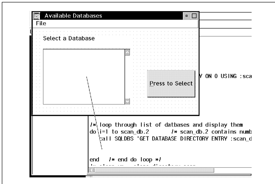
Figure 147. Drag ListBox Object
