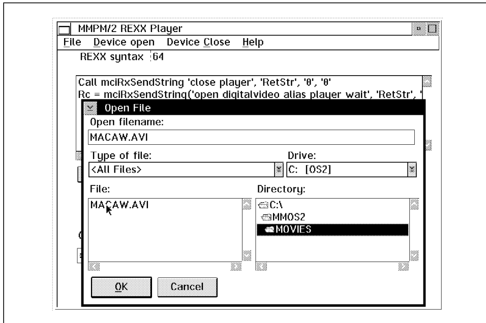
Figure 82. MPPM/2 REXX Player File Open
