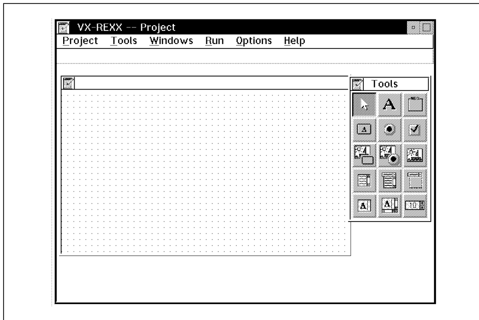
Figure 139. VX-REXX Initial Screen
