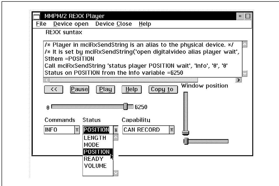
Figure 85. MPM/2 REXX Player Status List
