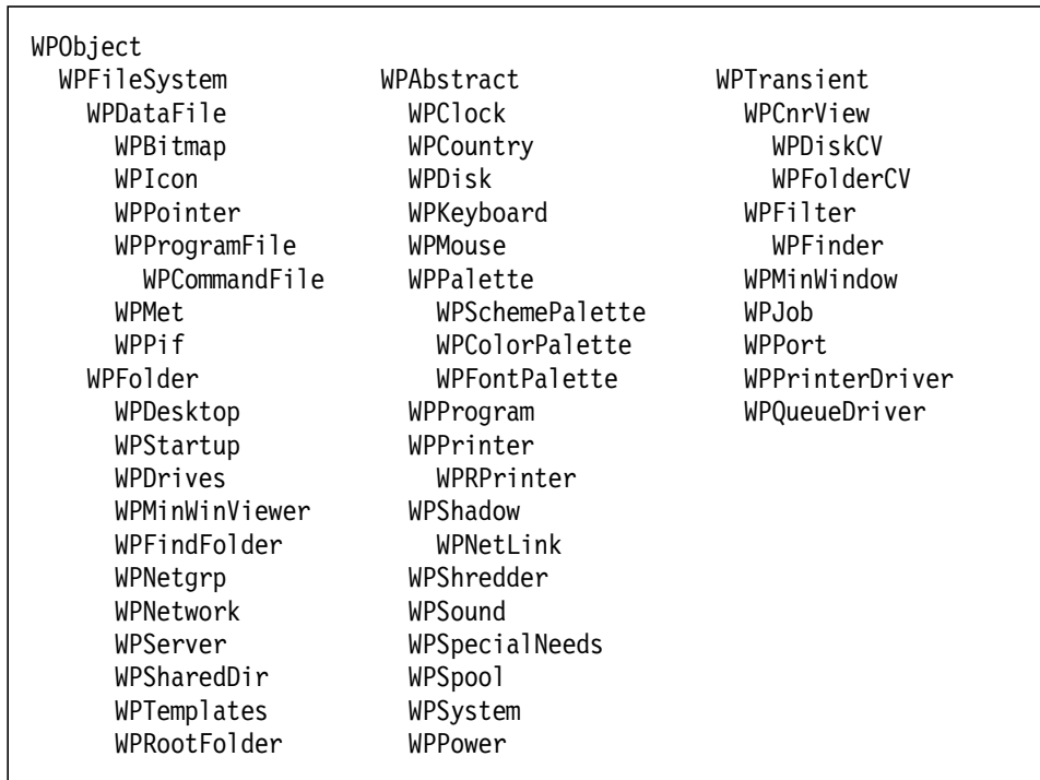
Figure 44. The Workplace Shell Object Class Hierarchy
