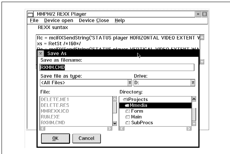
Figure 87. MPPM/2 REXX Player Save to File
