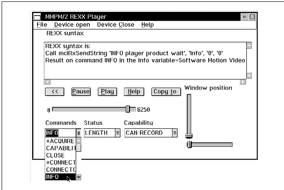
Figure 84. MPM/2 REXX Player Command List
