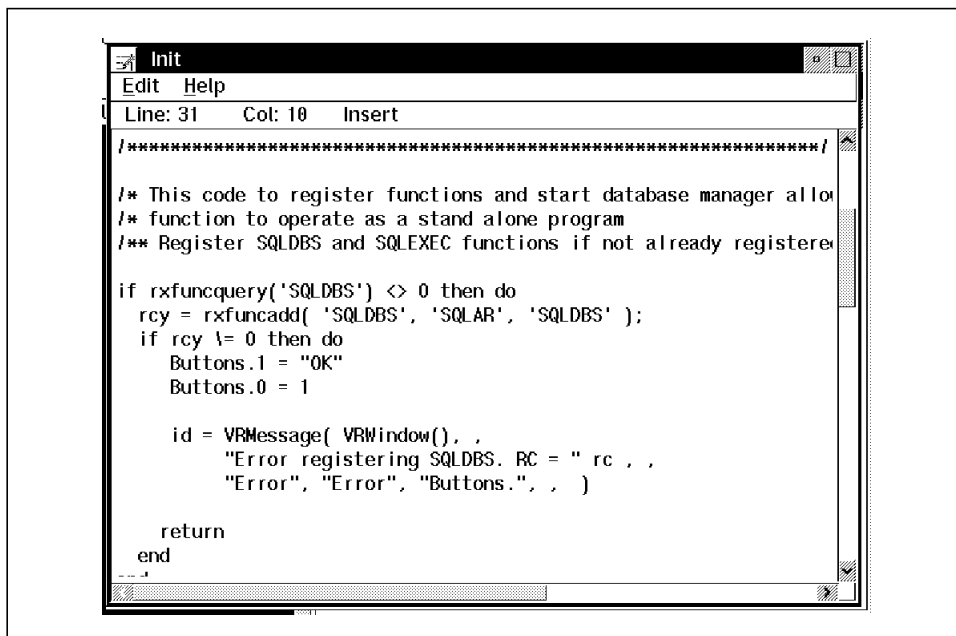
Figure 146. Message Box Code
