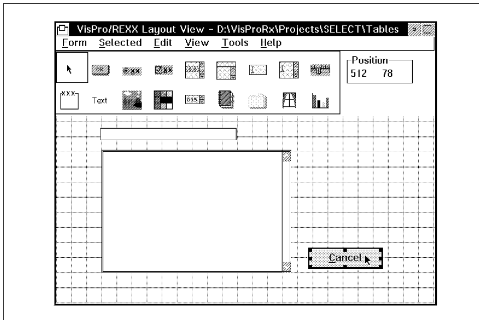
Figure 138. Tables Form in VisPro/REXX
