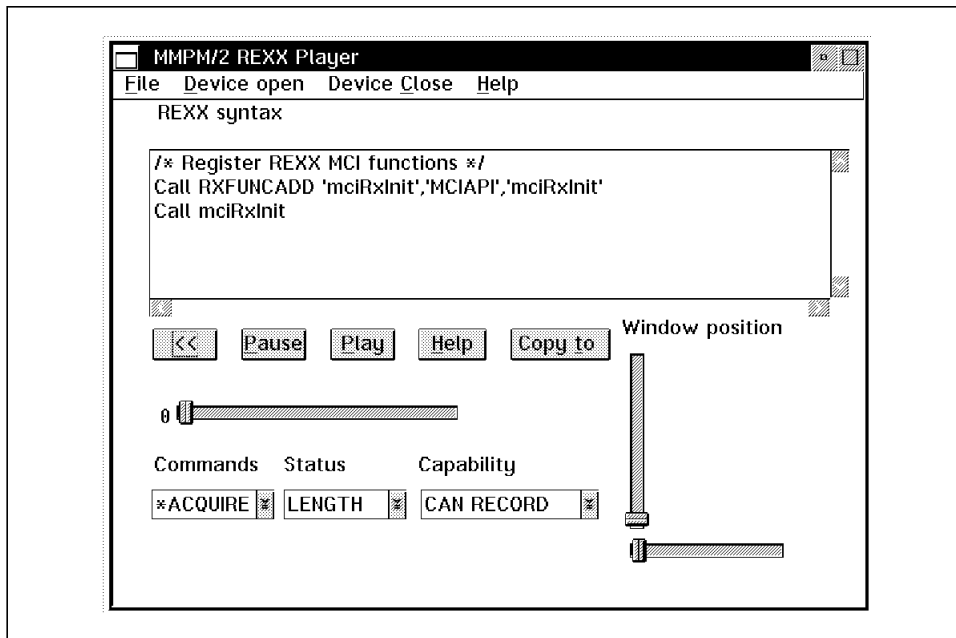
Figure 80. RXPLAY.EXE MPM/2 REXX Player
