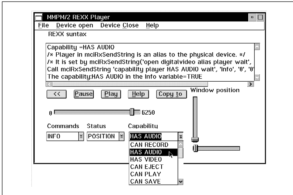
Figure 86. MPM/2 REXX Player Status List
