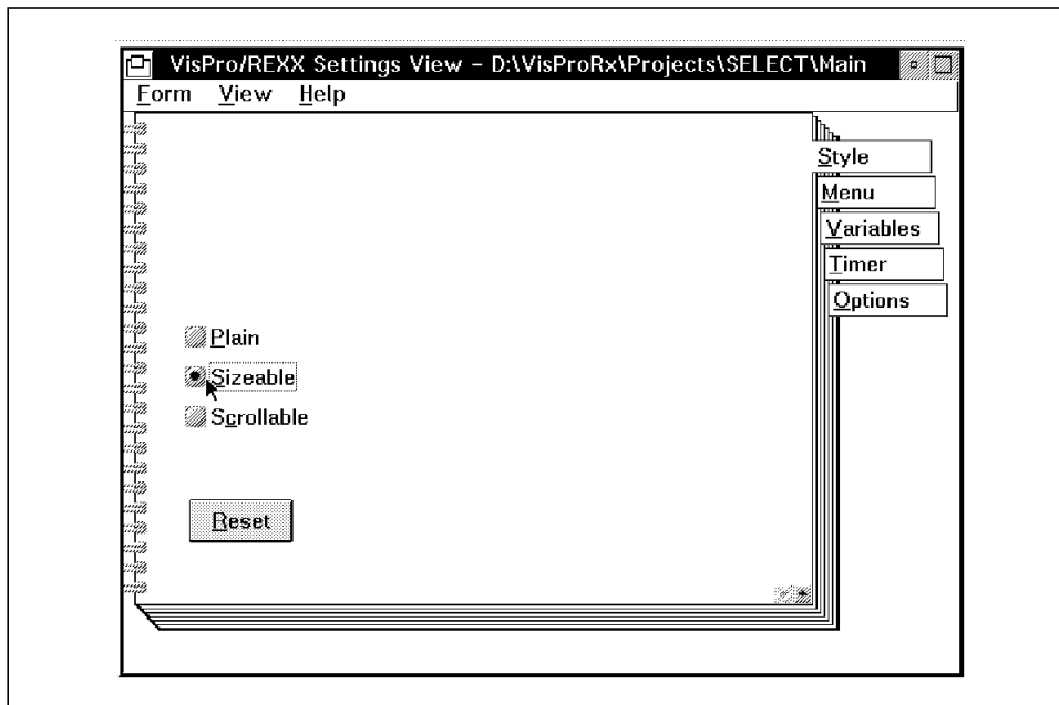
Figure 132. Form Settings Notebook in VisPro/REXX
