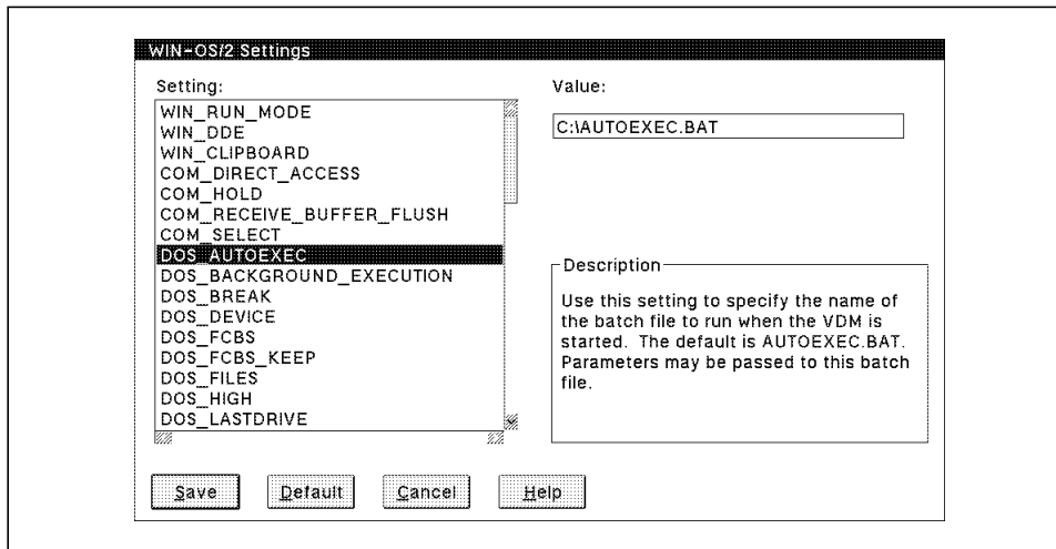
Figure 164. Settings Dialog on the Session Page of a Program Settings Notebook
