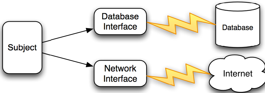
Figure 3—External dependencies
