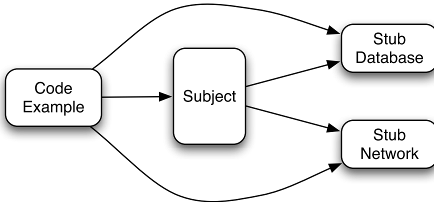
Figure 4—Stubbed dependencies
