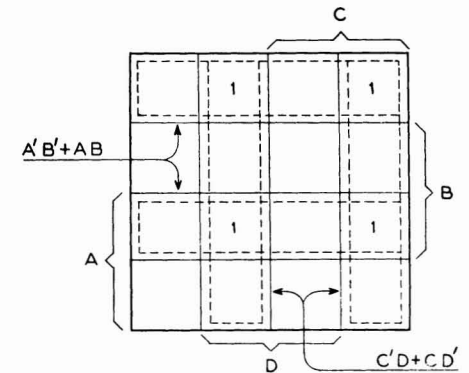
Fig. 9. Set theoretic interpretation of a map
