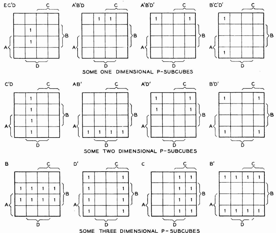
Fig. 5. A number of typical p -subcubes and the corresponding algebraic products
