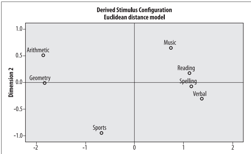
Figure 16-5. MDS common space mappings (Alscal)
