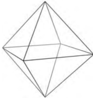
Figure 1.3 Triangle subdivision: starting octahedron.
