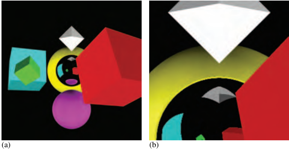
Figure 5.7 Example showing sparkle artifacts.
