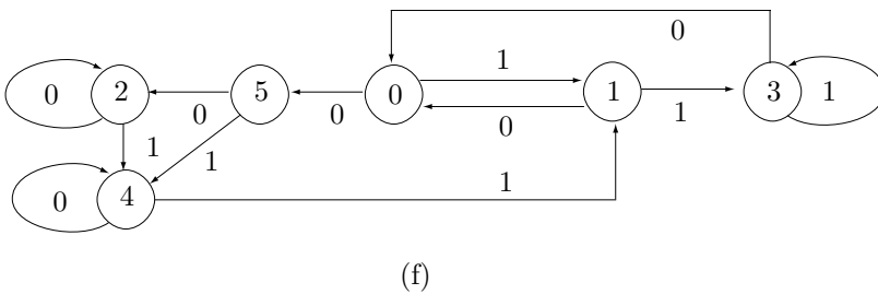
Figure 8.39: First Six States.
