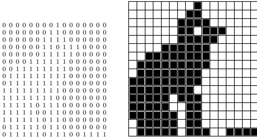
Figure 4.166: A 16 \times 16 Matrix M_0 .
