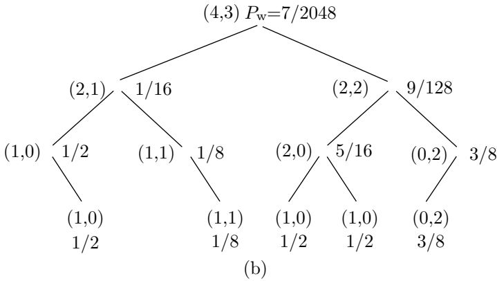
Figure 2.81: (a) A Context Tree. (b) A Weighted Context Tree.
