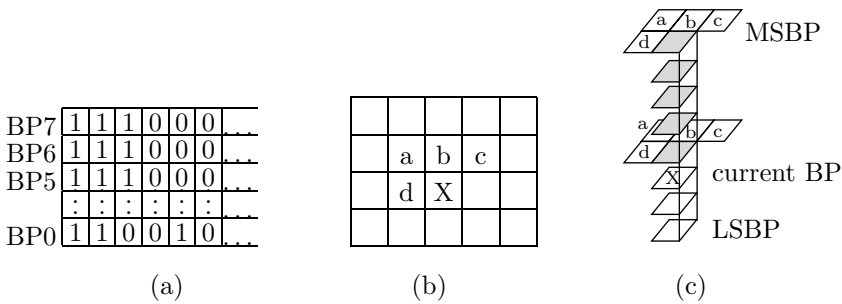
Figure 4.107: Pixel Contexts Used by EIDAC.
