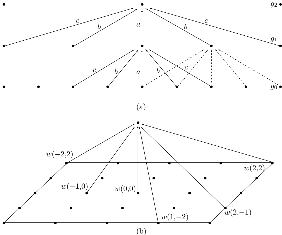
Figure 5.55: Illustrating Reduction.
