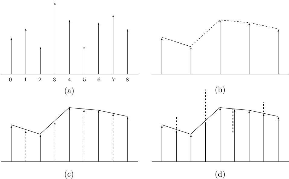
Figure 5.49: Linear Prediction.
