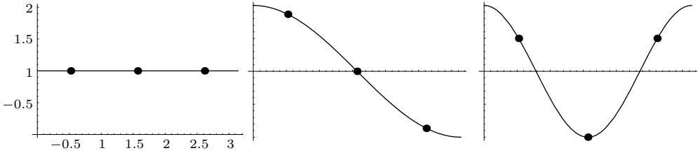
Figure 4.39: Increasing Frequencies.
