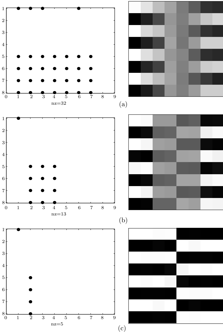
Figure 5.20: Three Lossy Reconstructions of an 8x8 Image.
