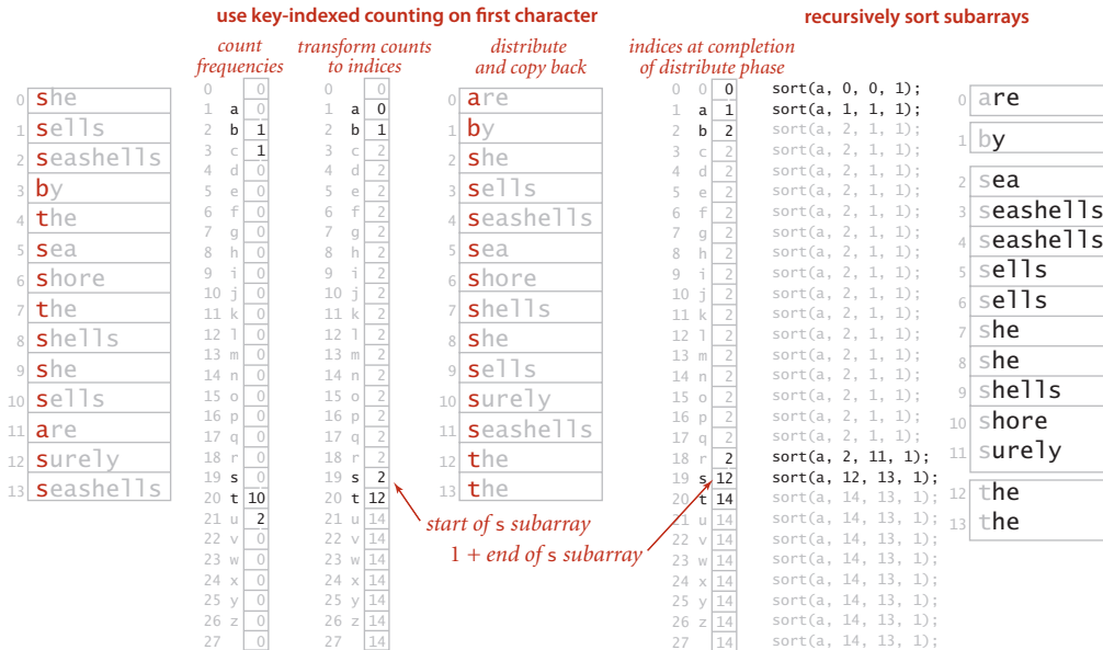
Trace of MSD string sort: top level of sort(a, 0, 14, 0)
