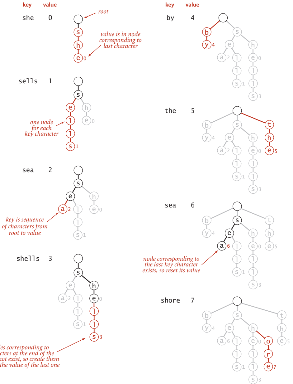
Trie construction trace for standard indexing client
