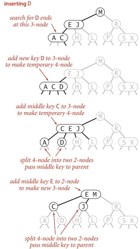
Insert into a 3-node whose parent is a 3-node
