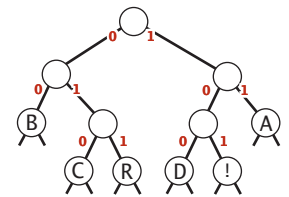
trie representation
