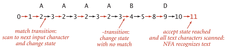
Finding a pattern with ((A*B|AC)D) NFA
