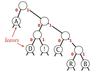
trie representation
