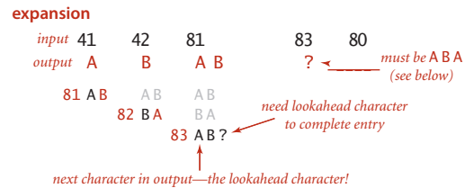
LZW expansion: tricky situation
